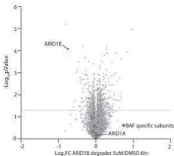
Figure 16. ARID1B degrader exhibits selective degradation as evidenced by global proteomics
